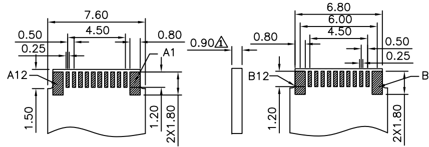
Recommended P.C.B. Layout (PCB Board Tolerance±0.05)
