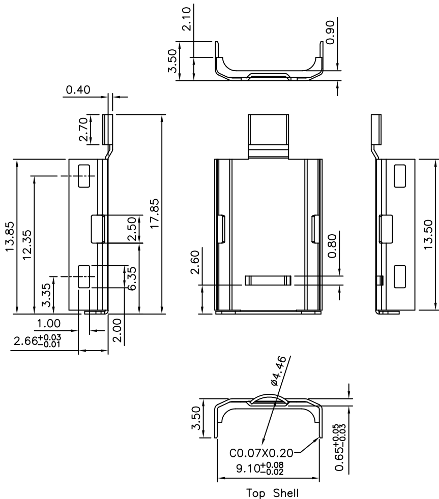
Top Shell
