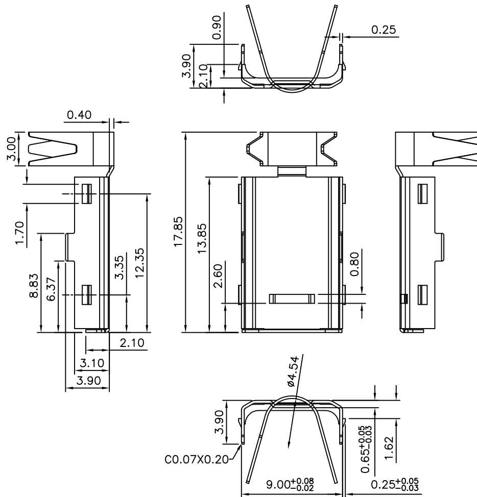
Bottom Shell
