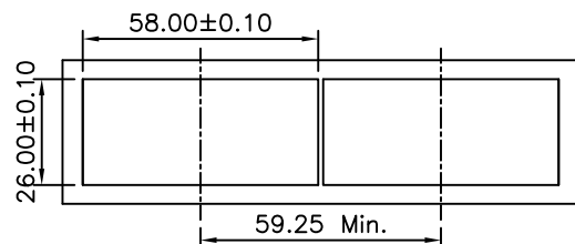
Bezel Cut-Out Center Spacing Detail Bezel Thickness:0.8~2.6
